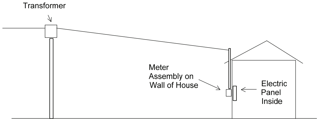
Overhead Service to Meter On Wall of House
